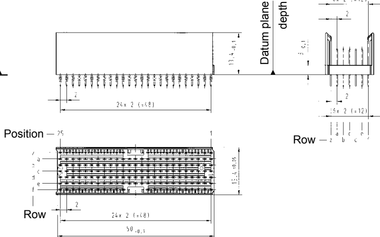
Connector dimensions [mm]
